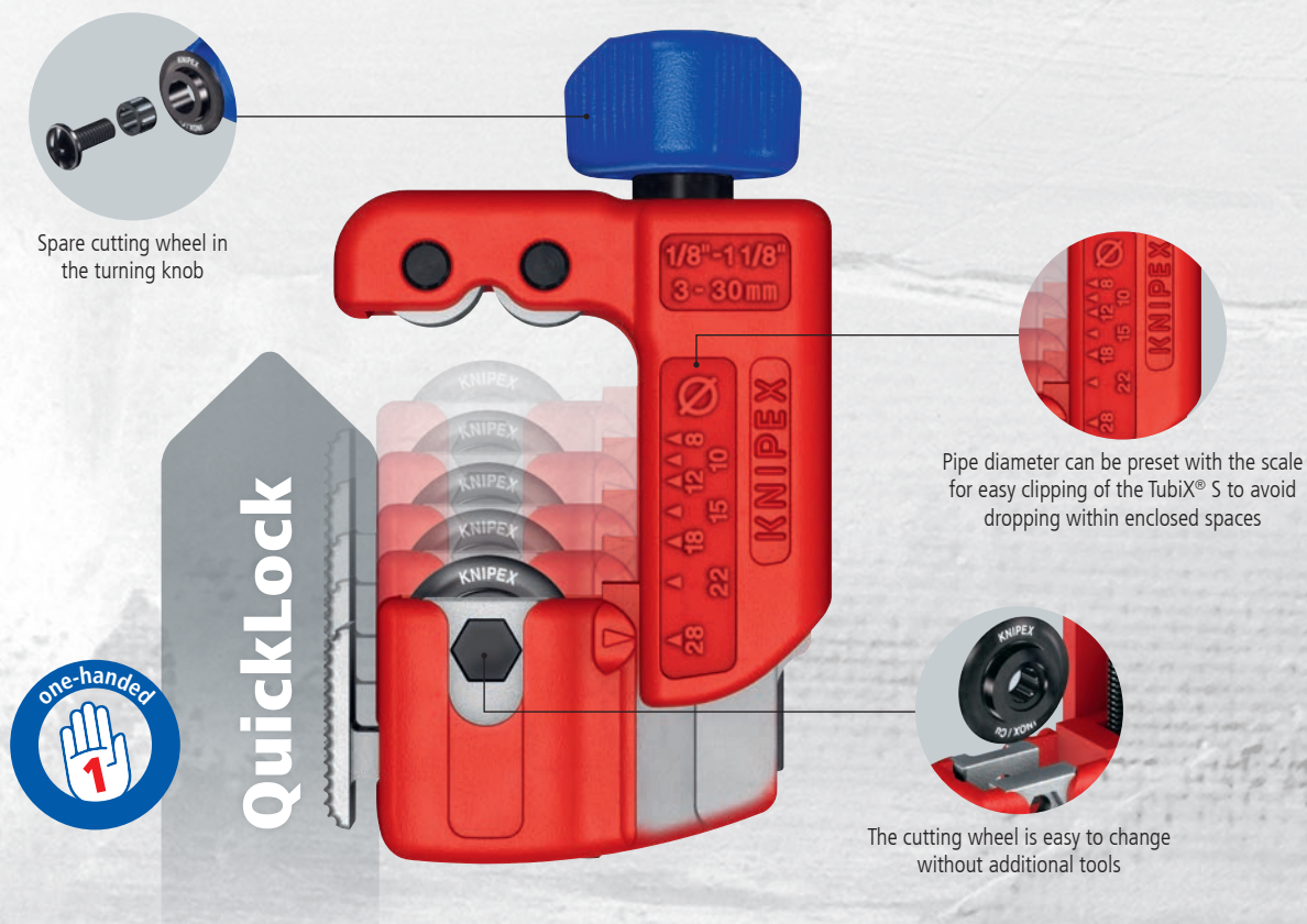
... preset with the scale and click onto the tube with the spring-loaded cutting wheel
